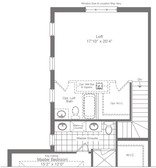
OPT. SECOND FLOOR Elev. C1 W/Loft
