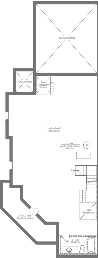
BASEMENT Elev. C1
