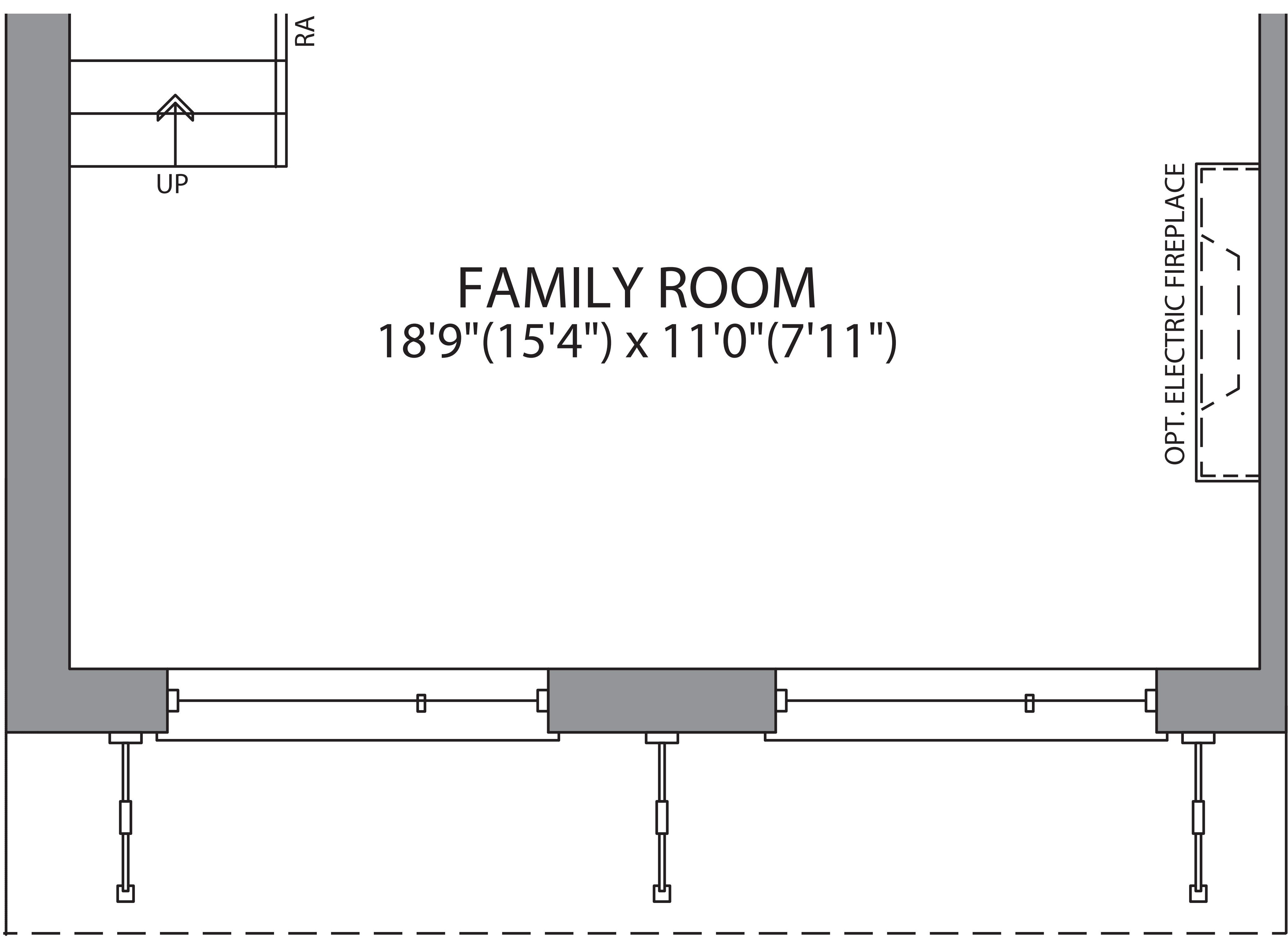
MAIN FLOOR PLAN ELEV. C-3
