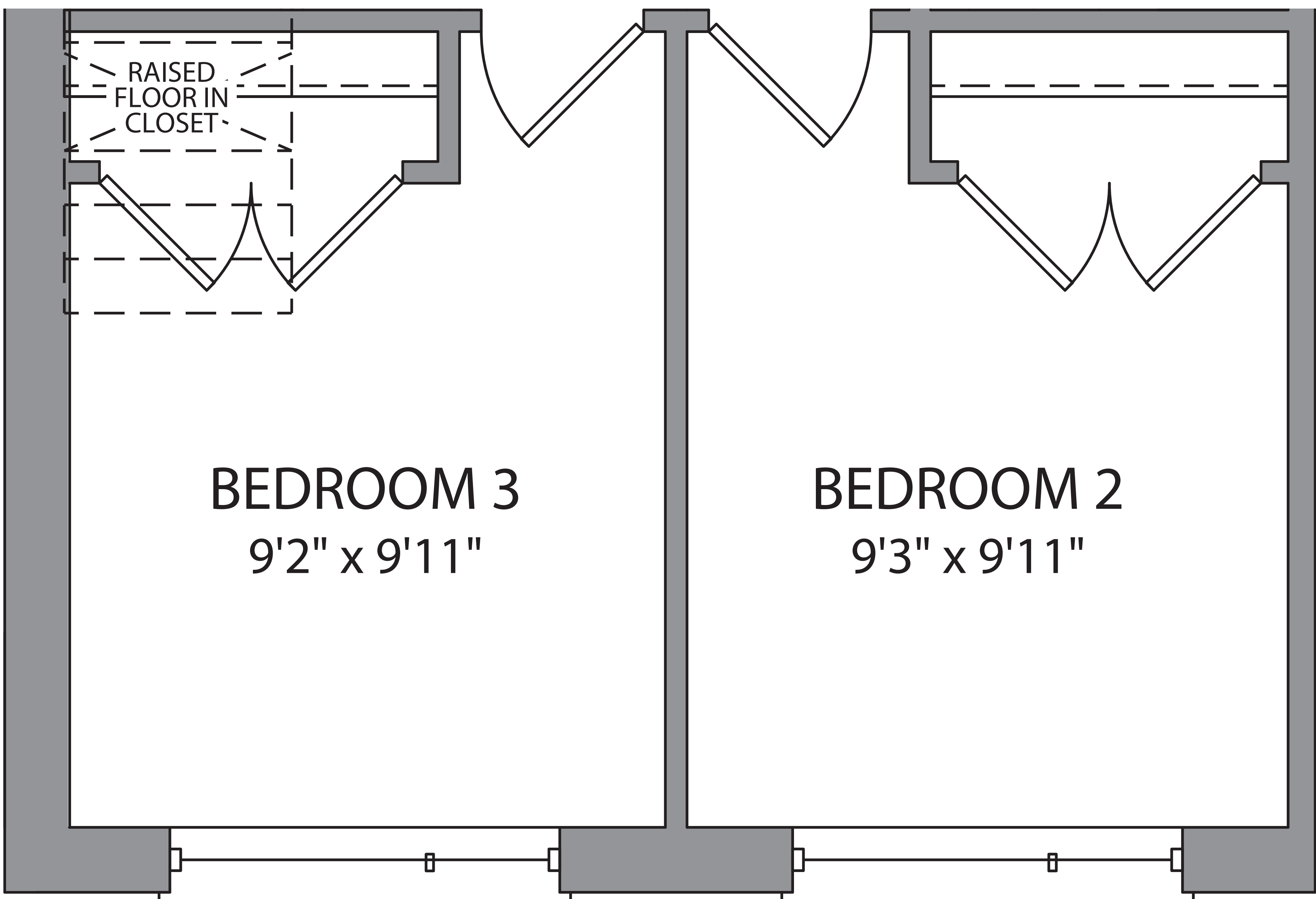
UPPER FLOOR PLAN ELEV. C-2
