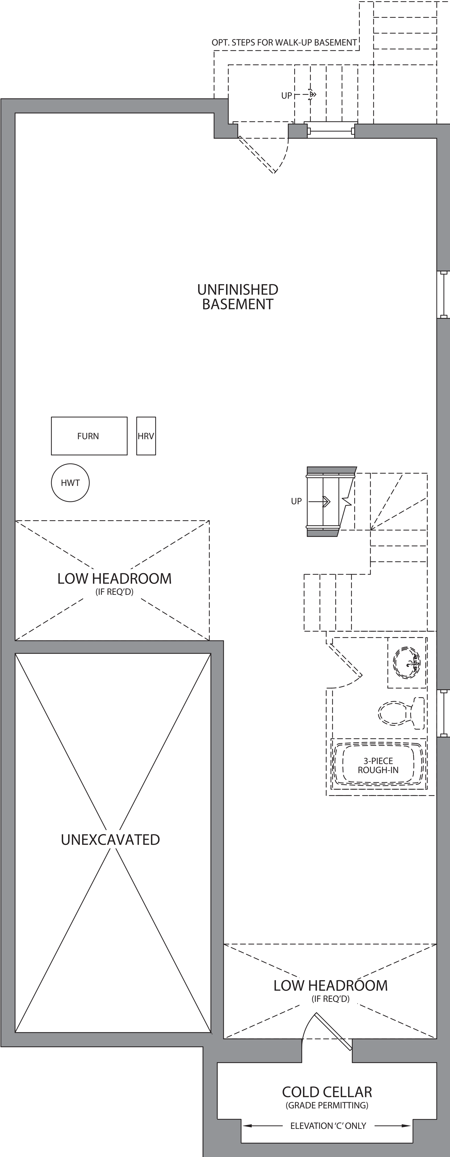
BASEMENT ELEV. T, C & F
