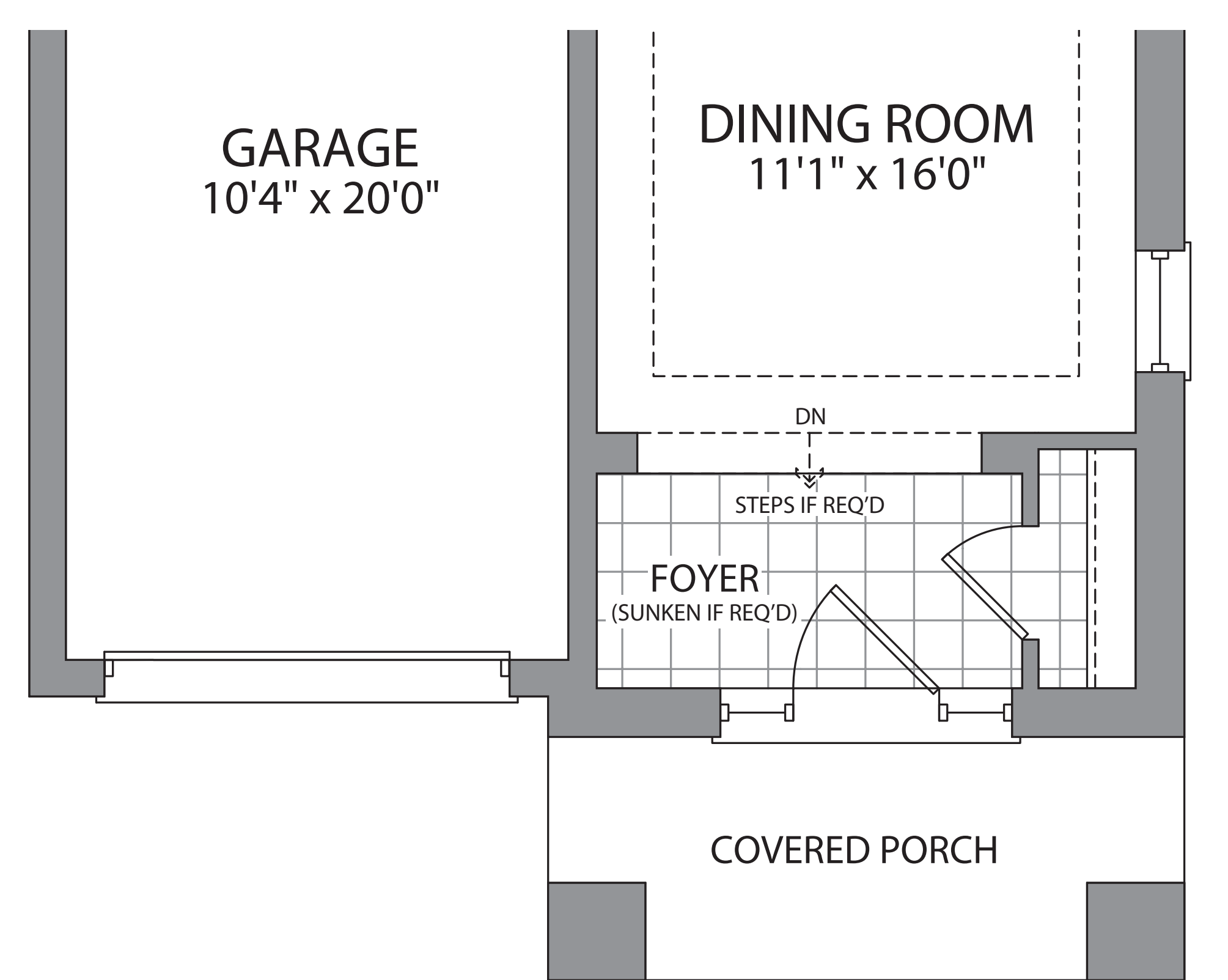
MAIN FLOOR ELEV. C
