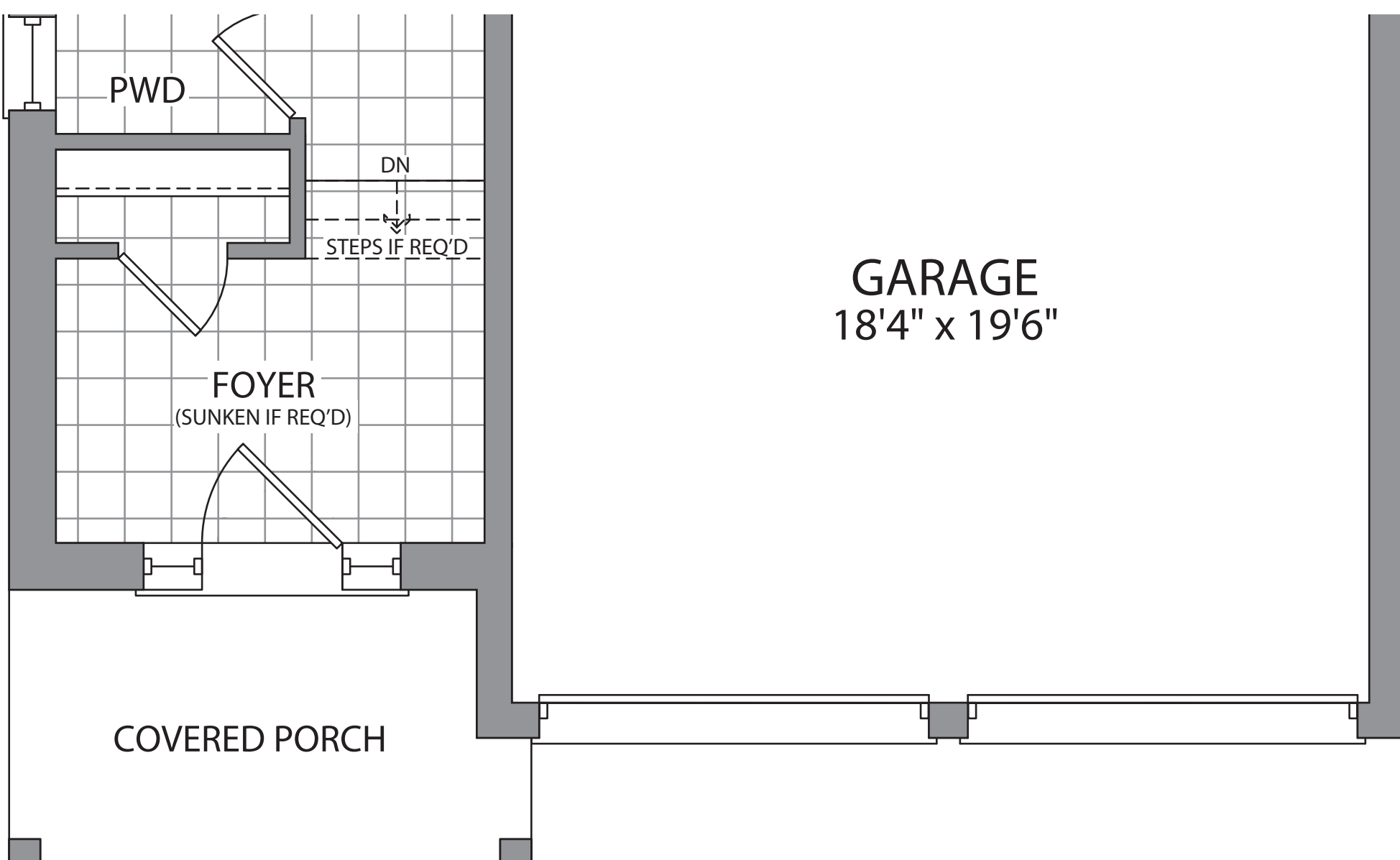
PART. MAIN FLOOR ELEV. F
