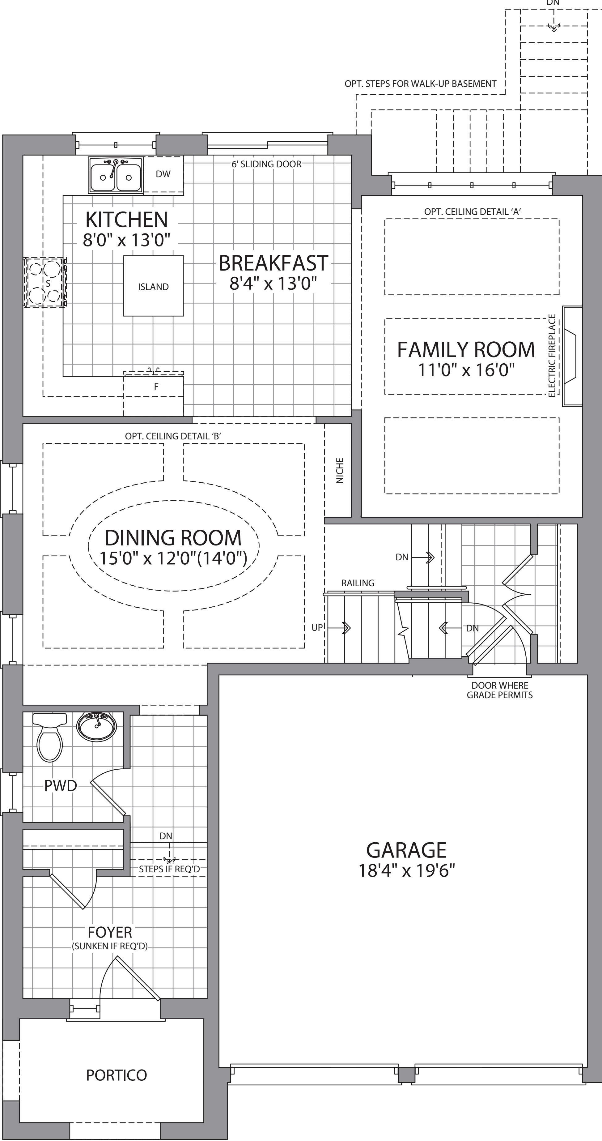
MAIN FLOOR ELEV. T
