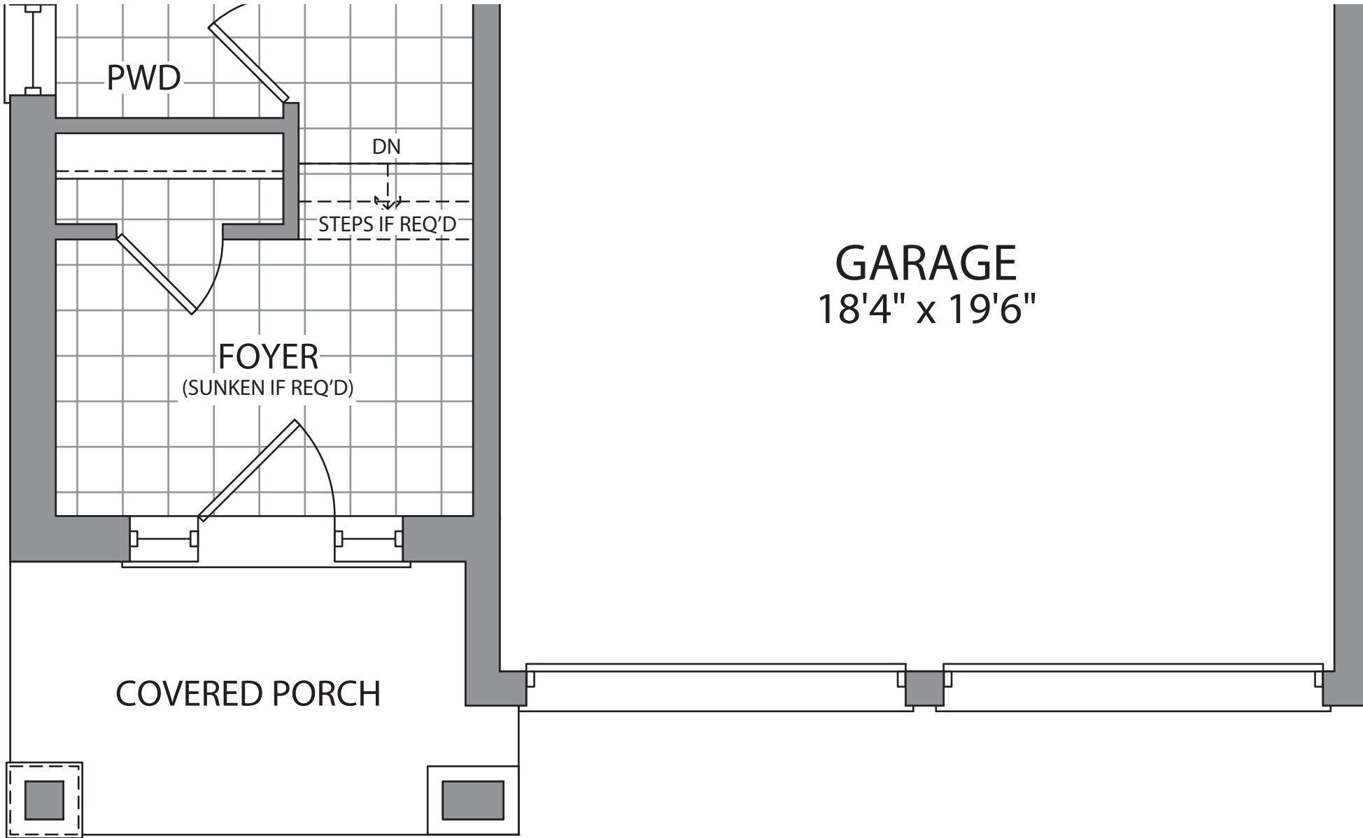
PART. MAIN FLOOR ELEV. C
