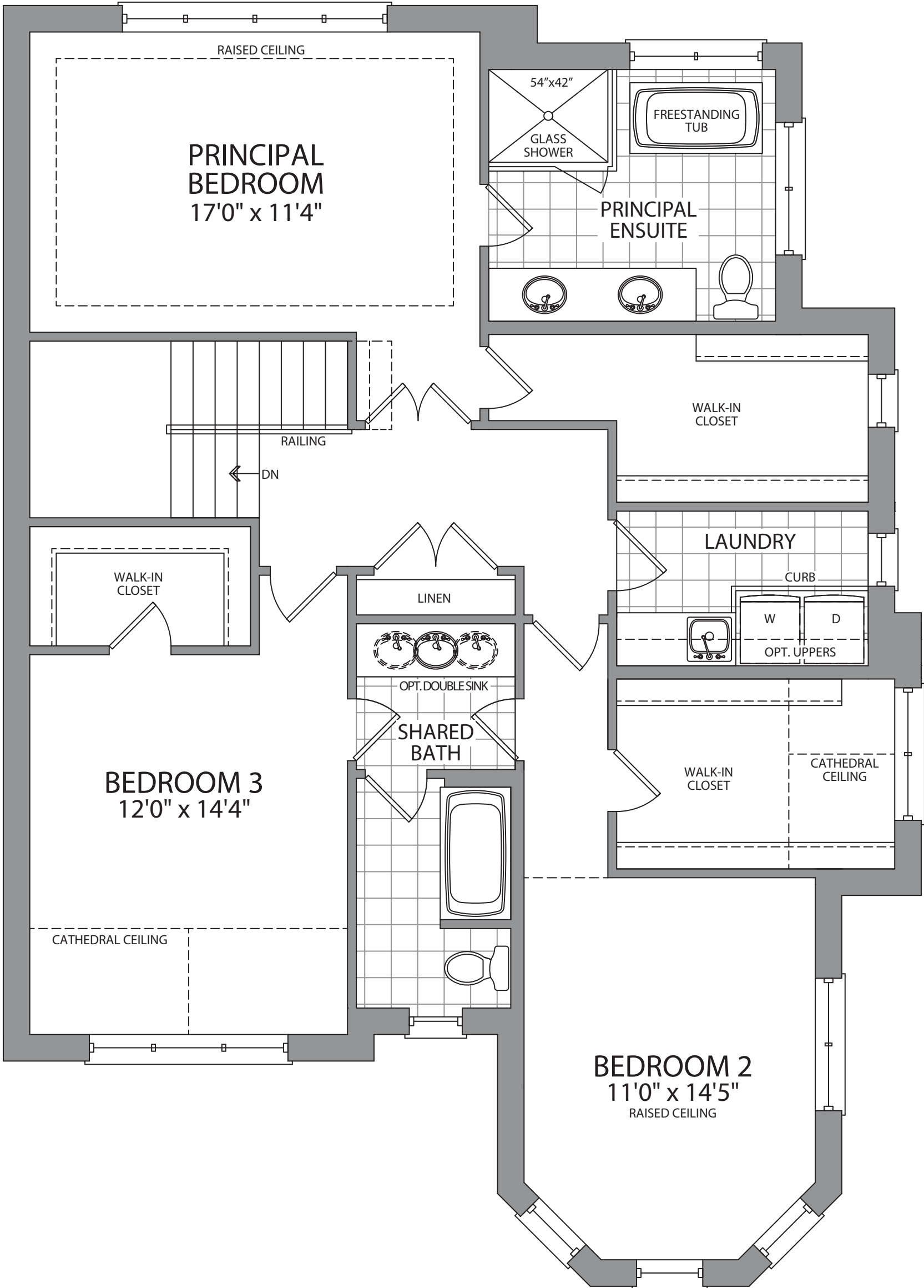
UPPER FLOOR ELEV. T
