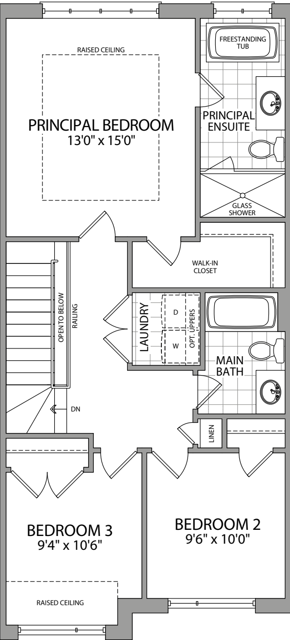
UPPER FLOOR ELEV. C
