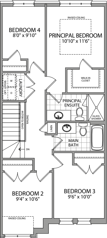
OPT. UPPER FLOOR 4 BEDROOM PLAN ELEV. F
