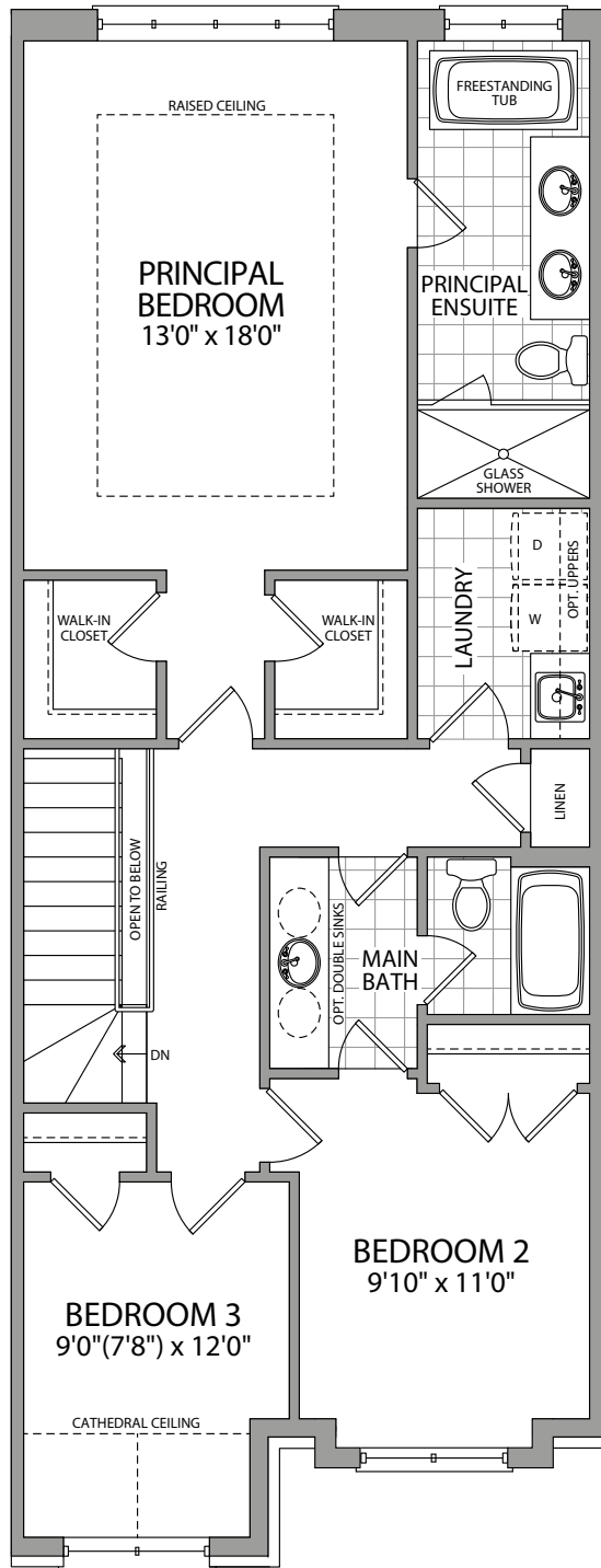
UPPER FLOOR ELEV. F
