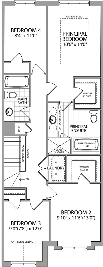
OPT. UPPER FLOOR 4 BEDROOM PLAN ELEV. F
