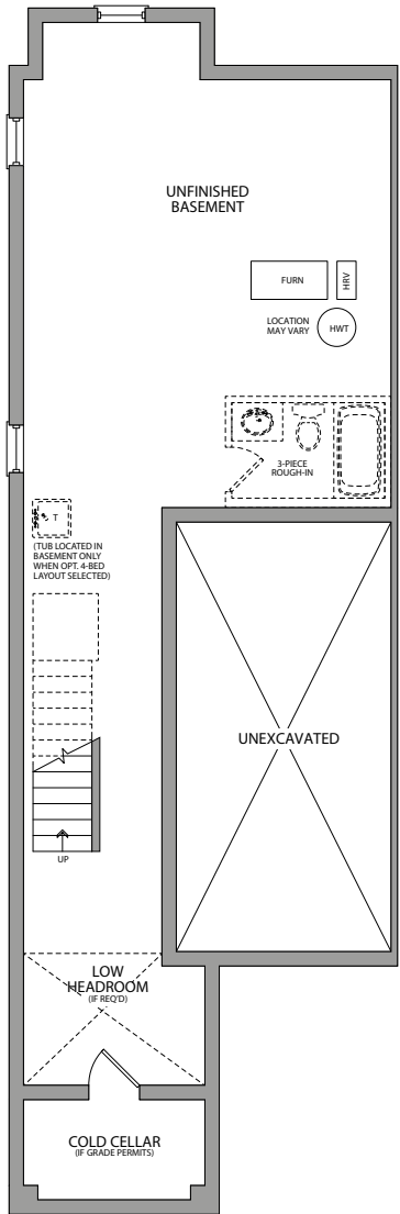
BASEMENT ELEV. C
