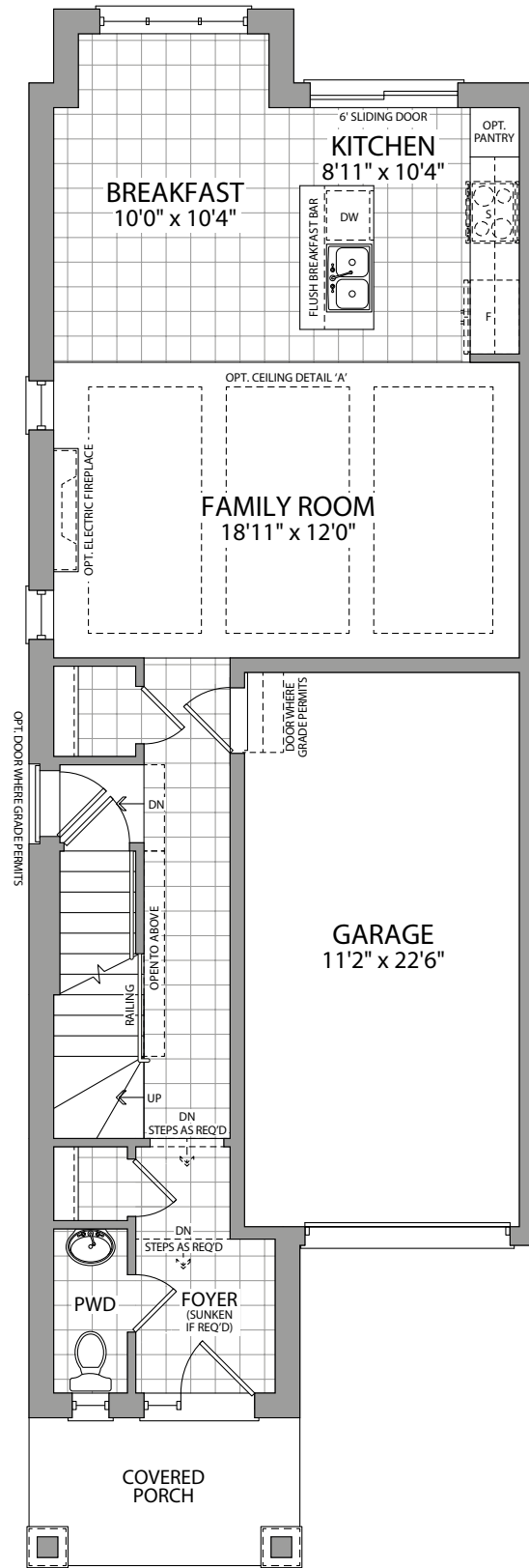
MAIN FLOOR ELEV. C
