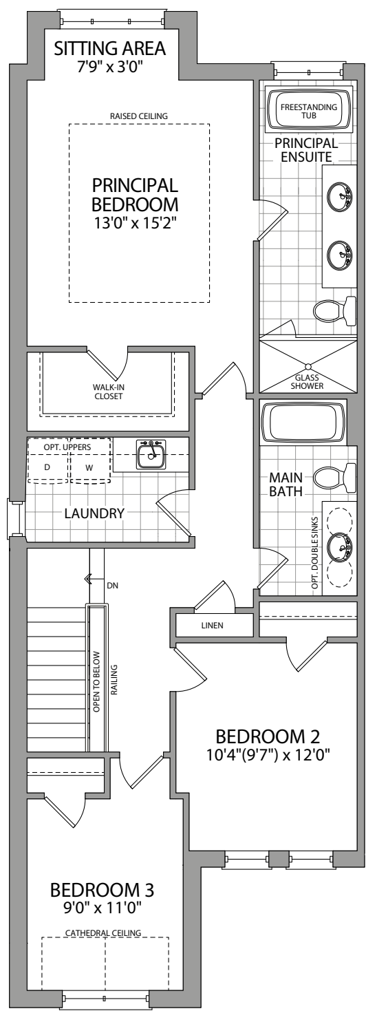
UPPER FLOOR ELEV. F
