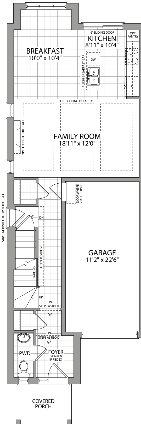
MAIN FLOOR ELEV. F
