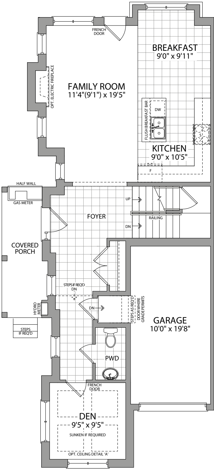
MAIN FLOOR ELEV. F
