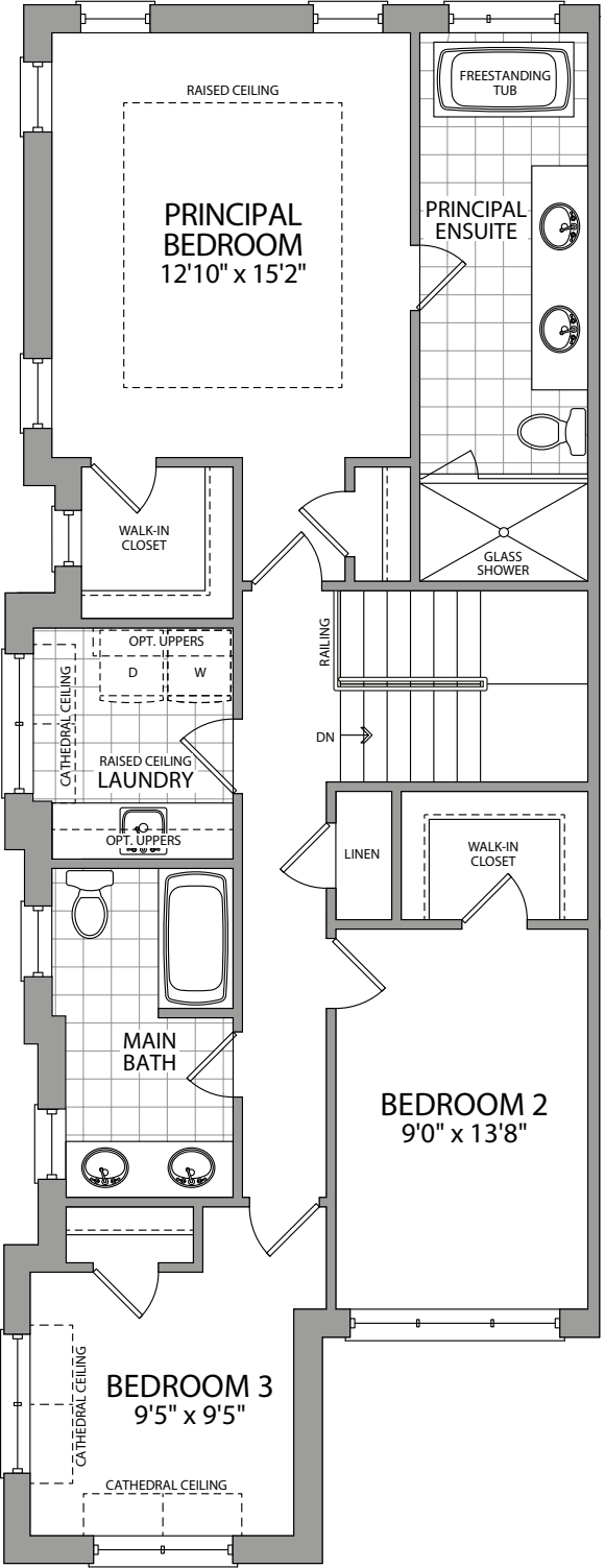
UPPER FLOOR ELEV. F
