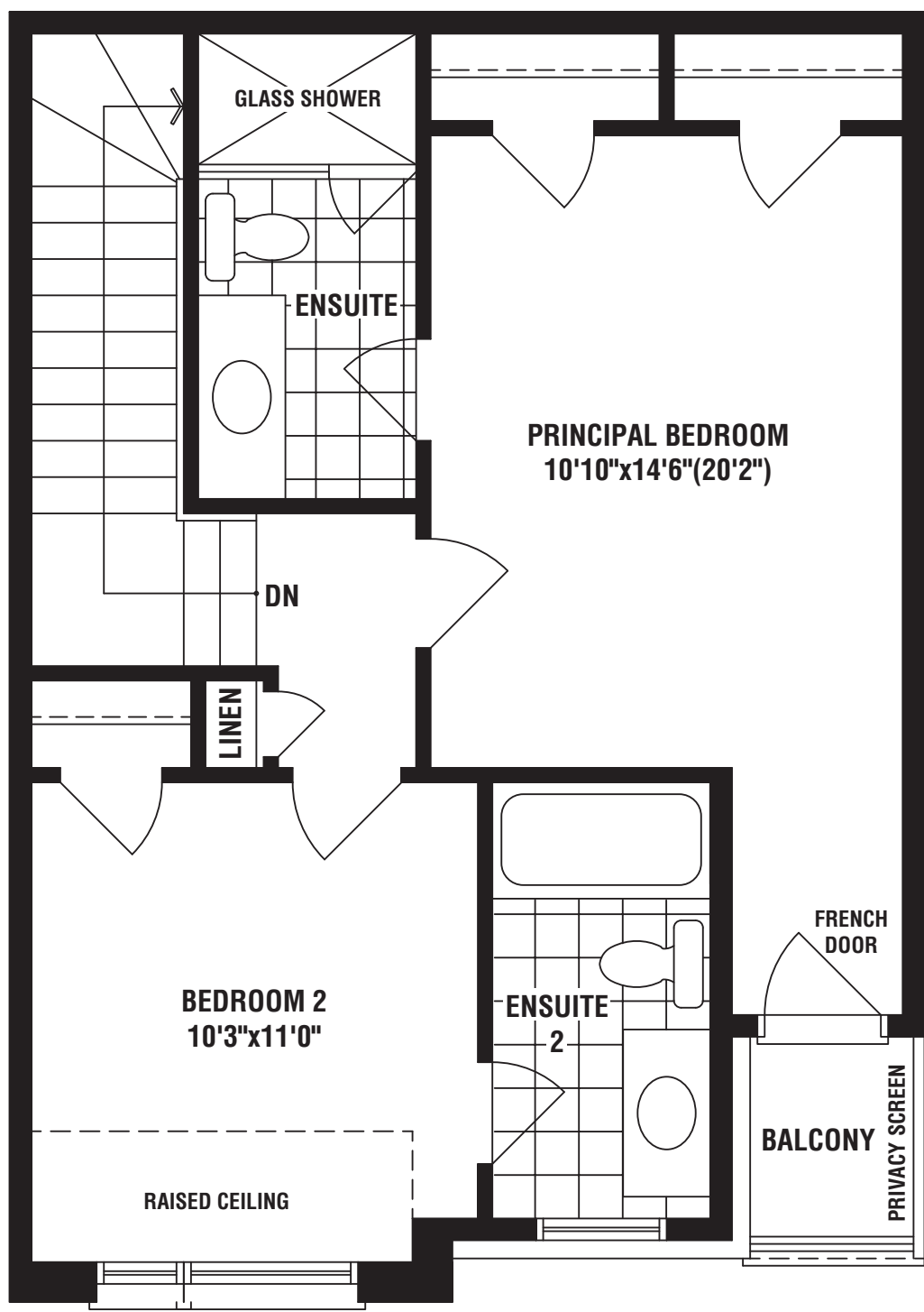
UPPER FLOOR ELEV. 'A'
