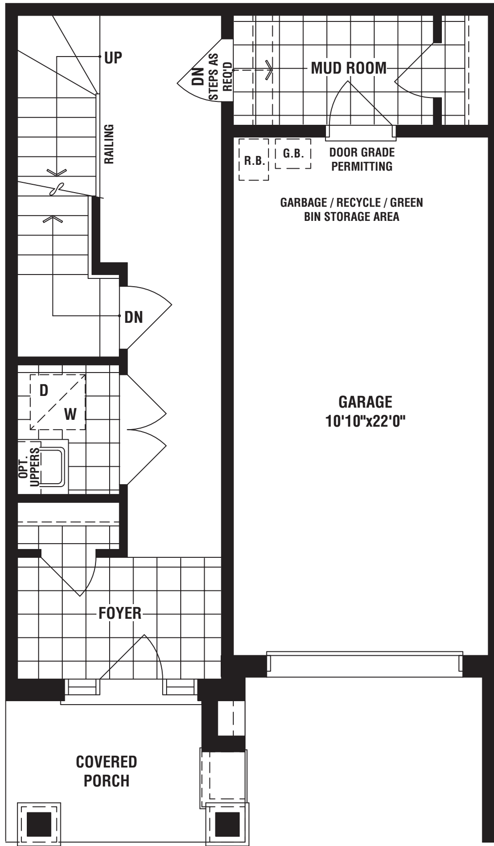
LOWER FLOOR ELEV. 'A'
